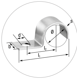
NORMAFIX® BSL TYPE 510 FOR 1 LINE (In accordance with DIN 72571)
