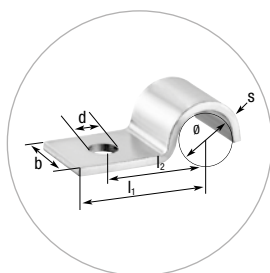
NORMAFIX® BSS TYPE 530 FOR 1 LINE
