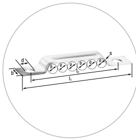
NORMAFIX® BSL TYPE 512 FOR 6 LINES (In accordance with DIN 72573)
