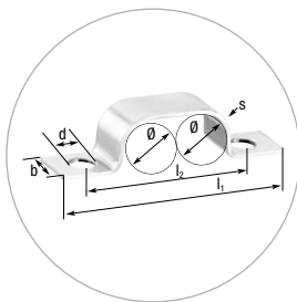
NORMAFIX® BSL TYPE 512 FOR 2 LINES (In accordance with DIN 72573)
